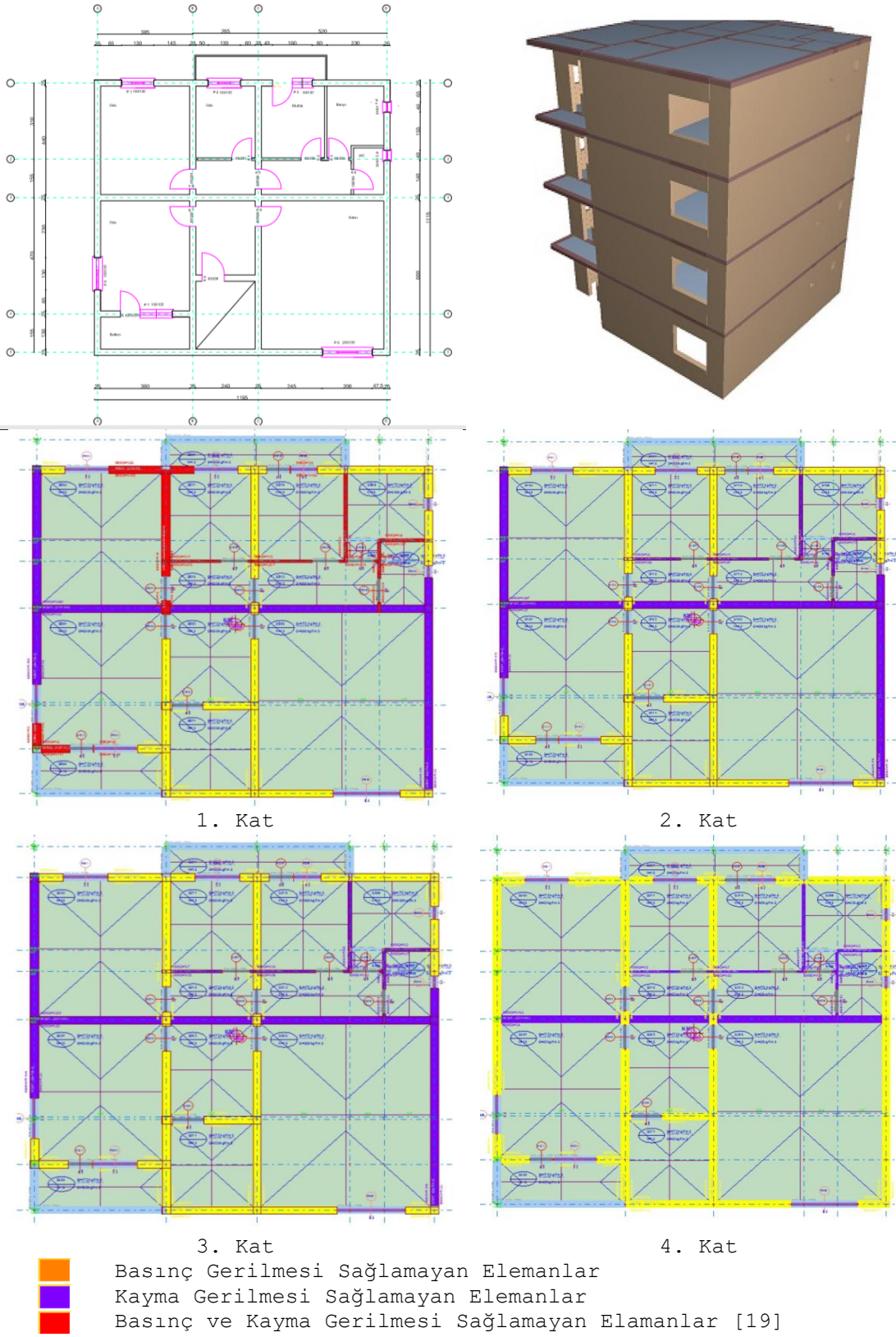
Şekil 6. YBÖ4 StaticallyCAD-Masonry bina risk analizi verileri (Figure 6. YBÖ4 StaticallyCAD-Masonry building risk analysis data)
