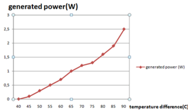
Figure 5. The power generated by the temperature difference of the Peltier
