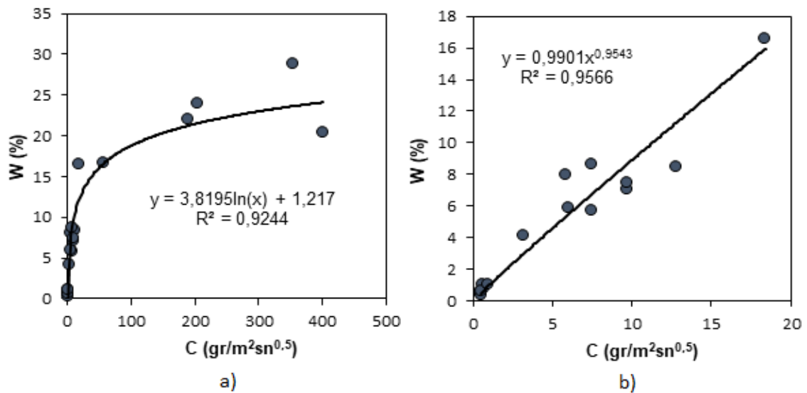
Figure 4. The relationship between water absorption properties of rocks (a-total specimens, b-except for high water absorption specimens)
