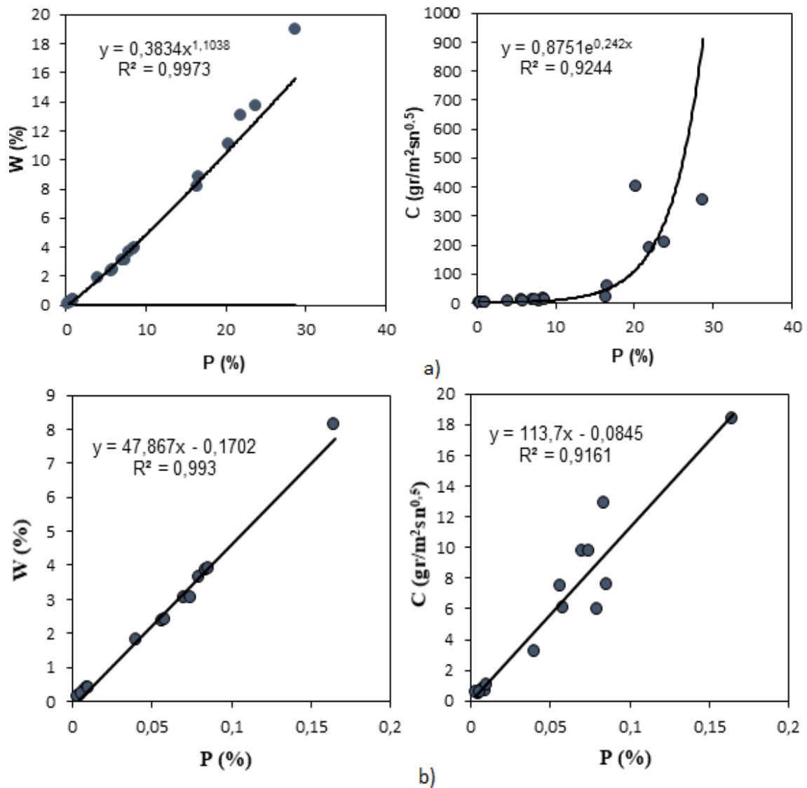
Figure 3. Water absorption properties (a-total specimens and b-except for high water absorption specimens) versus porosity
