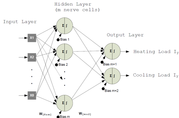
Figure 2. YSA Forecast Model
