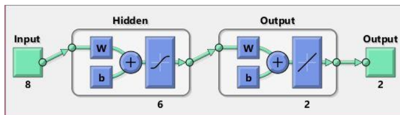
Figure 3. Developed YSA model for implementation
