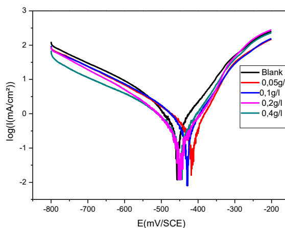
Figure 2. Polarization curves of mild steel in 1 M HCl at 35°C containing different concentrations of LM extract
