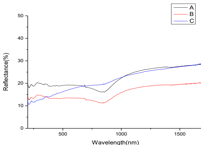
Figure 7. UV spectrum for aluminum specimens in 1M HCl solution in the absence and presence of 0.1g/l of LM extract as corrosion inhibitor: (A) before immersion, (B) immersion in 1M HCl, (C)with LM inhibitor
